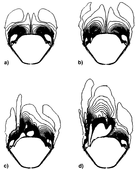
Fig. 10 Computed helicity density contours at f_x = 1.0 ; M_\infty = 0.2 , \alpha = 40 deg, Re_d = 2.81 \times 10^5 : a) no-blowing, b) region I, MFR = 0.23 \times 10^{-3} ; c) region II, MFR = 1.49 \times 10^{-3} ; d) region III, MFR = 4.17 \times 10^{-3} .
