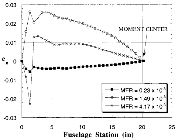
Fig. 8 Distribution of computed sectional yawing-moment coefficient along the body; M_\infty = 0.2 , \alpha = 40 deg, Re_d = 2.81 \times 10^5 .
