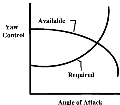
Fig. 1 Yaw control power.
