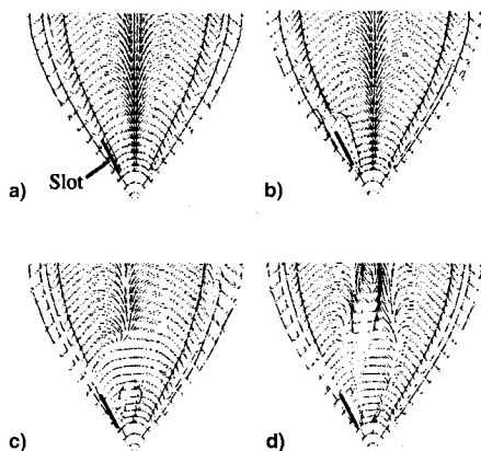
Fig. 9 Computed surface flow patterns; M_\infty = 0.2 , \alpha = 40 deg, Re_d = 2.81 \times 10^5 : a) no-blowing; b) region I, MFR = 0.23 \times 10^{-3} ; c) region II, MFR = 1.49 \times 10^{-3} ; and d) region III, MFR = 4.17 \times 10^{-3} .
