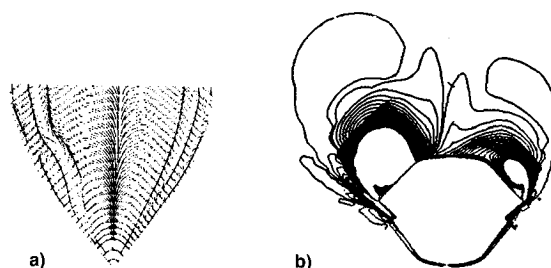
Fig. 14 Computed surface flow pattern and helicity density contours for bottom-slot blowing; M_\infty = 0.2 , \alpha = 40 deg, Re_d = 2.81 \times 10^5 , MFR = 1.49 \times 10^{-3} ; a) surface flow pattern and b) helicity density contours, f_s = 1.0 .
