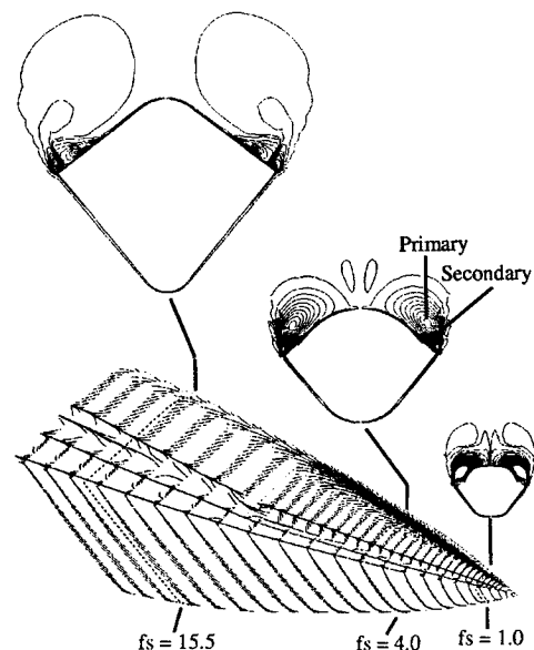
Fig. 5 Computed surface flow patterns and helicity density contours; no-blowing, M_\infty = 0.2 , \alpha = 40 deg, Re_d = 2.81 \times 10^5 .
