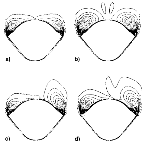
Fig. 7 Computed helicity density contours at fuselage station, f_s = 4.0 ; M_\infty = 0.2 , Re_d = 2.81 \times 10^5 : a) no-blowing, \alpha = 30 deg; b) no-blowing, \alpha = 40 deg; c) MFR = 1.49 \times 10^{-3} , \alpha = 30 deg; and d) MFR = 1.49 \times 10^{-3} , \alpha = 40 deg.
